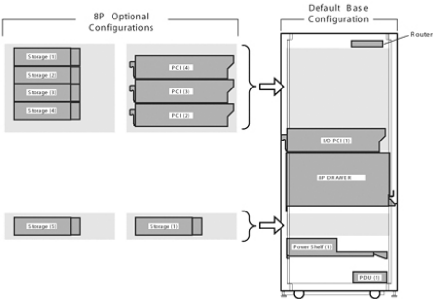
AlphaServer GS1280 Model 8 - Internal System Expansion Options
