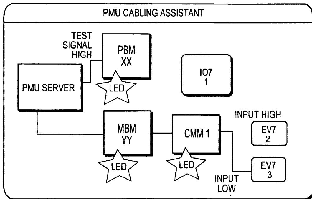
PMU CABLING ASSISTANT BLOCK DIAGRAM
