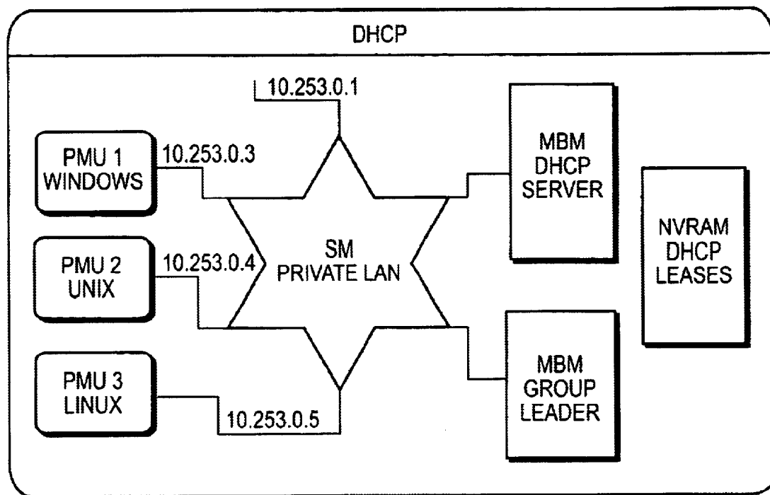
DHCP BLOCK DIAGRAM
