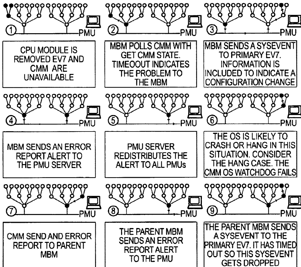
EV7 FAILYRE/REPLACE FLOW DIAGRAM (PART 1)
