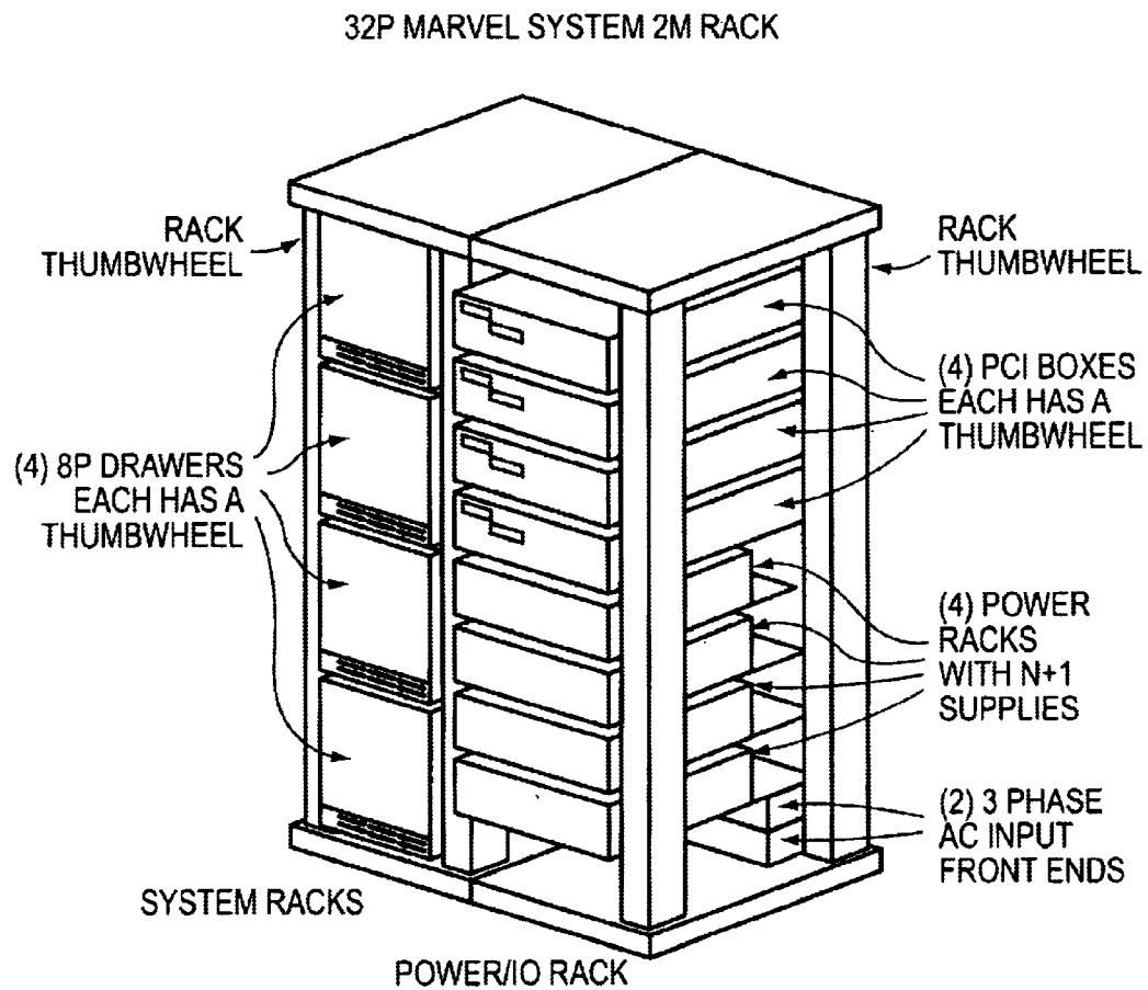
RACK AND BOX THUMBWHEEL SCHEME
