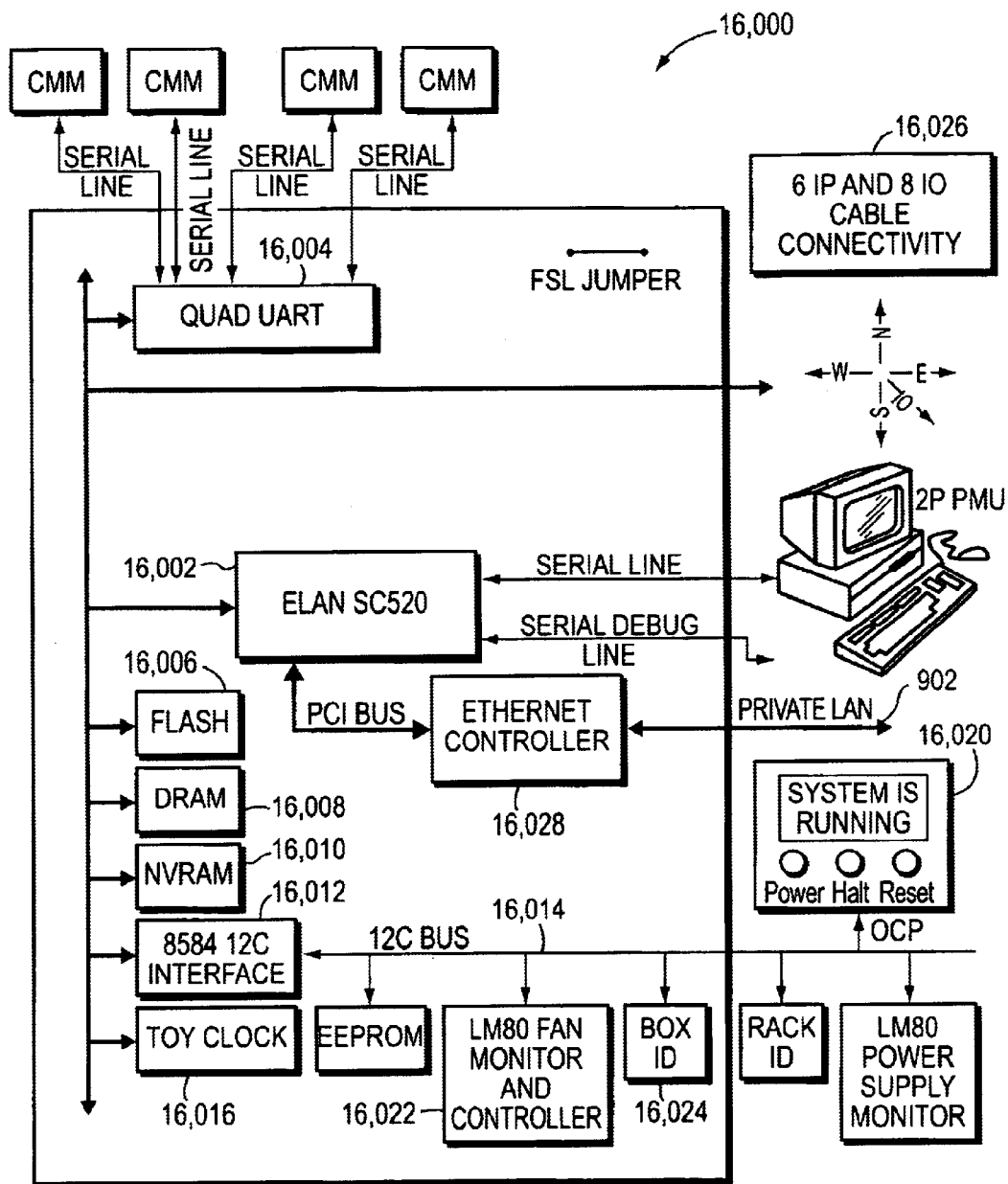
MBM HARDWARE OVERVIEW
