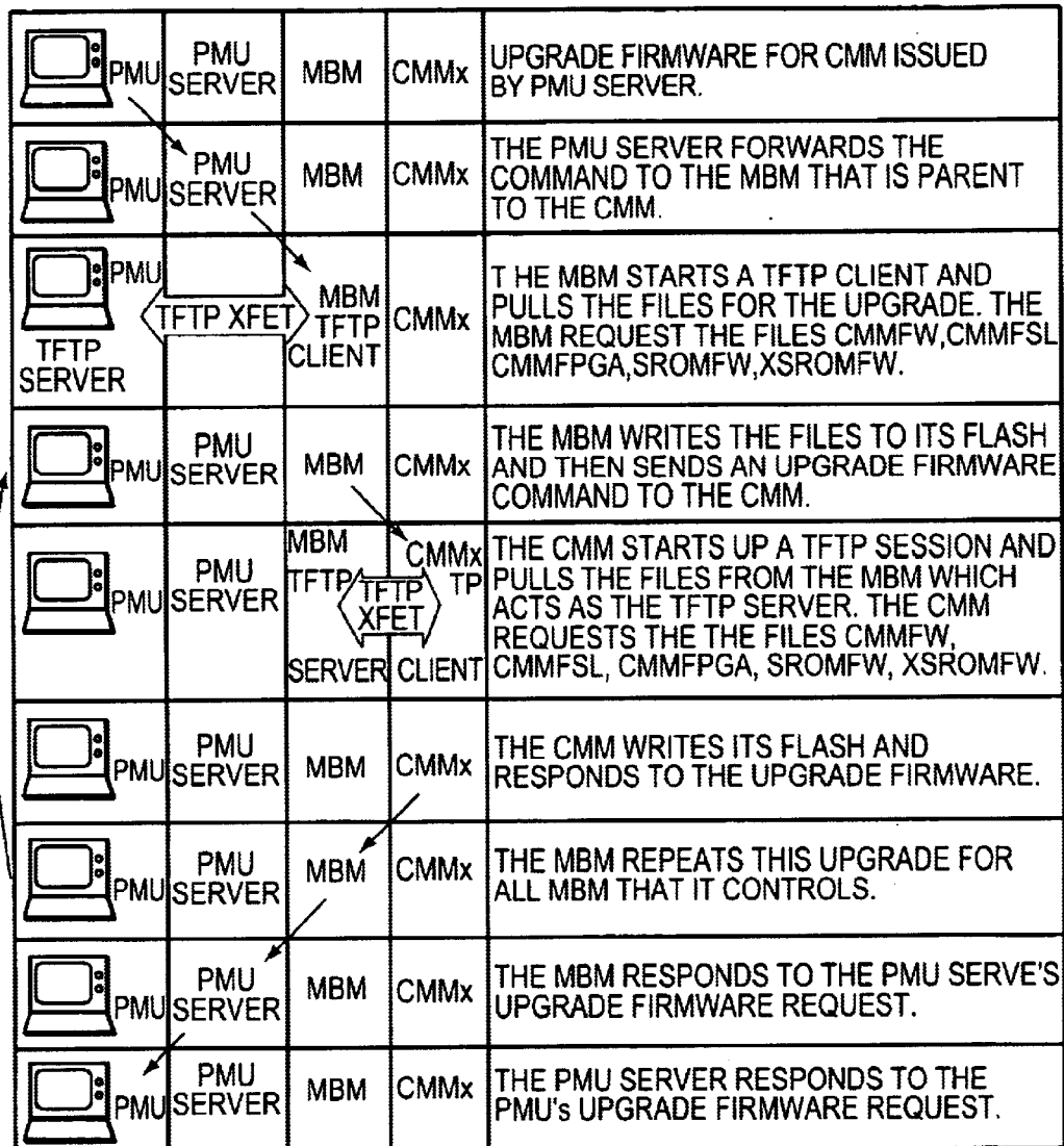
UPGRADING CMM FIRMWARE FLOW DIAGRAM
