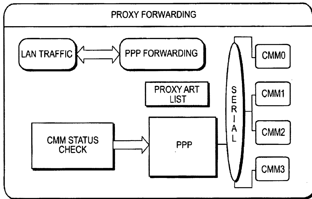
PROXY FORWARDING BLOCK DIAGRAM
