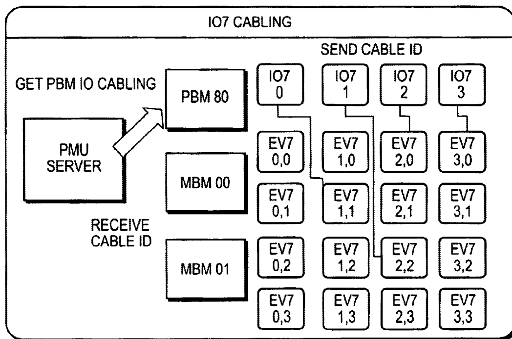
IO7 CABLING BLOCK DIAGRAM
