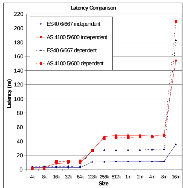
Figure 11 – Load Latency (and Bandwidth) Comparison
