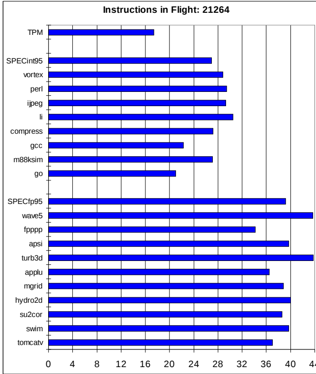
Figure 7 – Average Instructions in Flight
