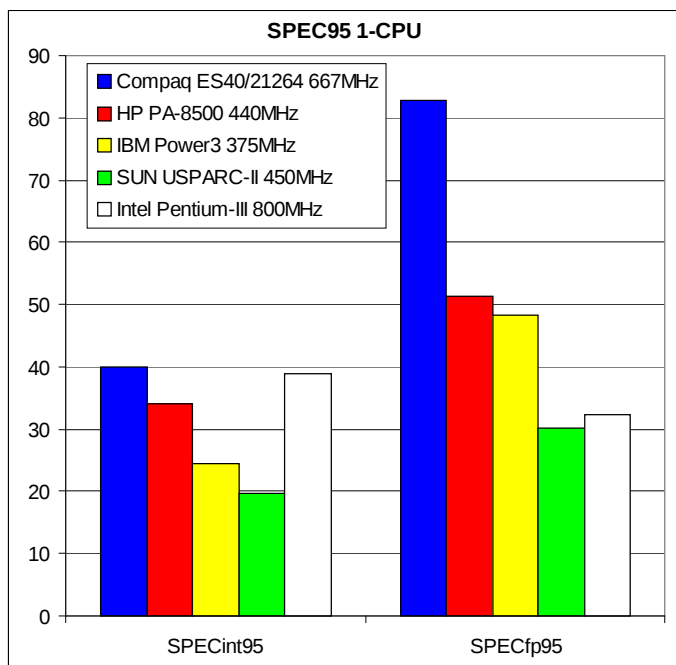
Figure 1 - SPEC95 Comparison
