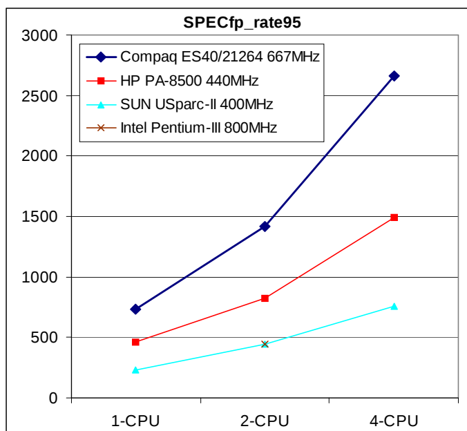
Figure 2 - SPECfp_rate95 Comparison
