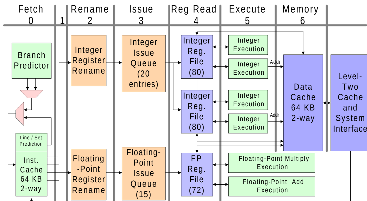
Figure 3 – The Basic Alpha 21264 Instruction Pipeline
