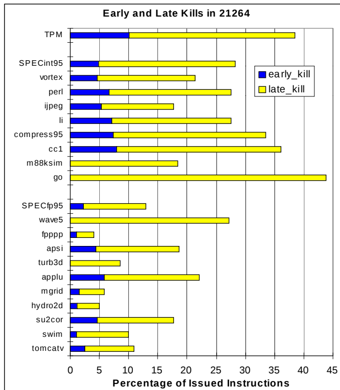
Figure 9 – Non-retired Instructions
