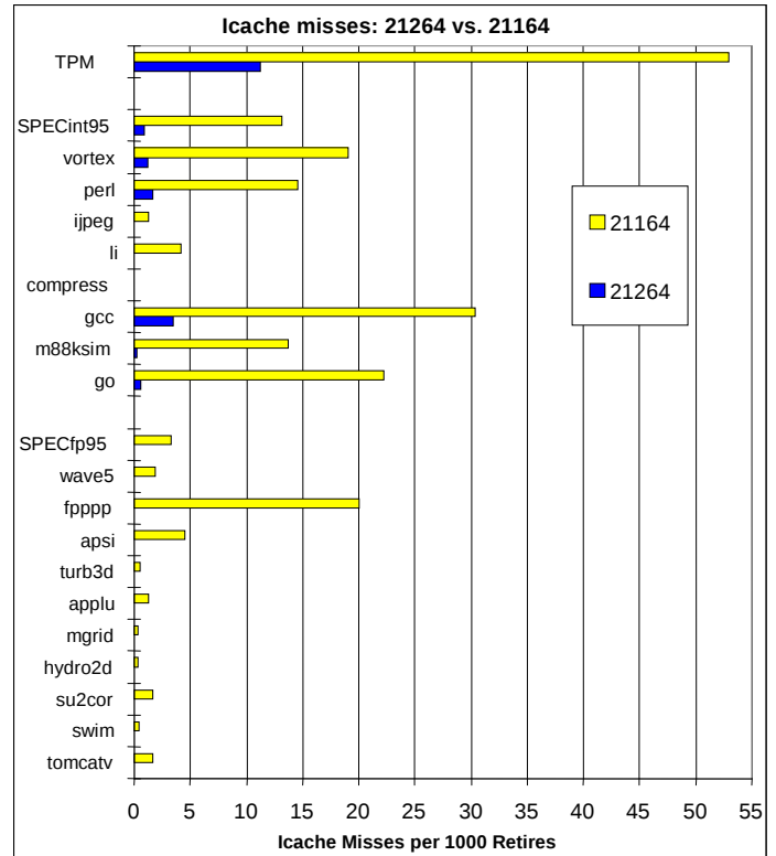
Figure 5 – Instruction Cache Miss Rate Comparison
