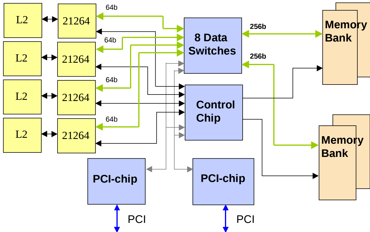
Figure 4 – ES40 Block Diagram
