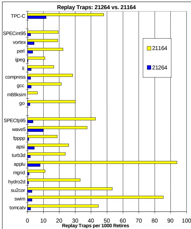
Figure 12 – Replay Trap Comparison
