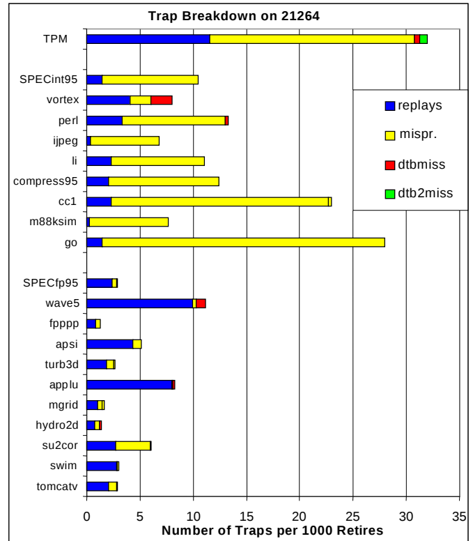
Figure 13 – 21264 Trap Breakdown
