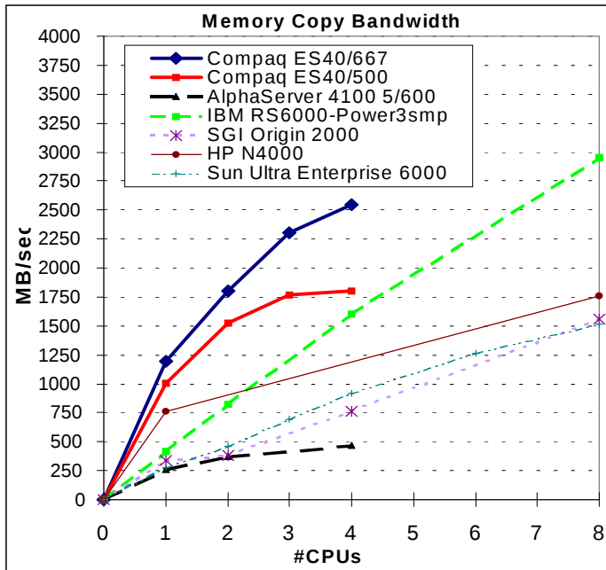
Figure 10 – STREAM Copy Bandwidth
