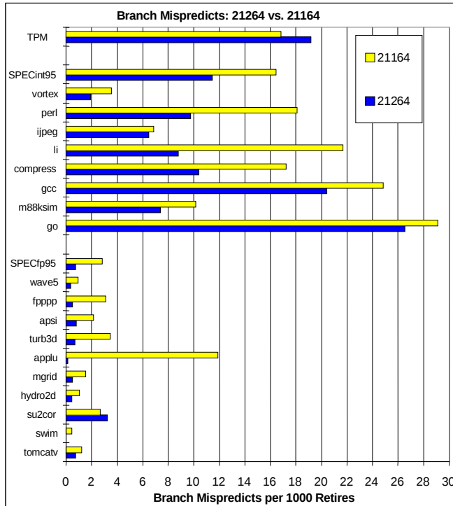
Figure 6 – Branch Mispredicts Comparison
