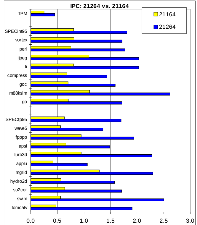
Figure 8 – IPC Comparison
