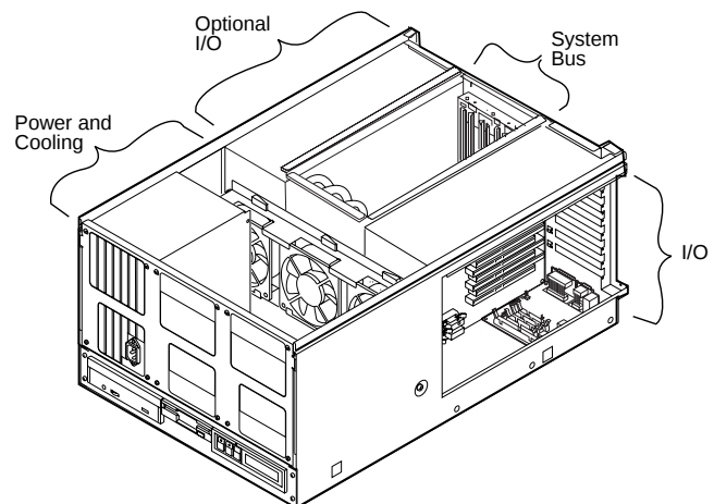
AlphaServer 4000 System Drawer
