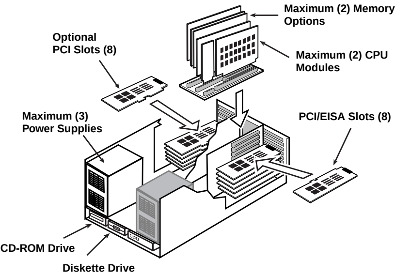
AlphaServer 4000 System Drawer
