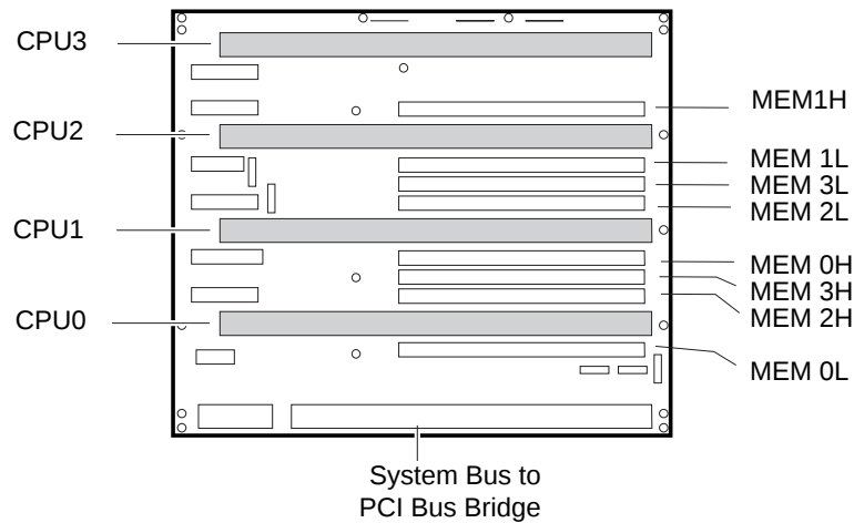
AlphaServer 4100 Motherboard
