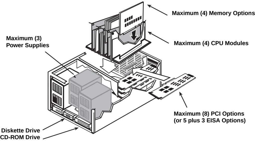
AlphaServer 4100 System Drawer
