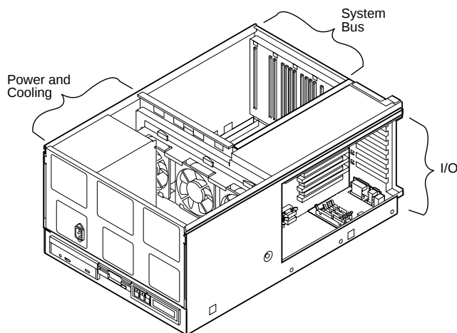
AlphaServer 4100 System Drawer
