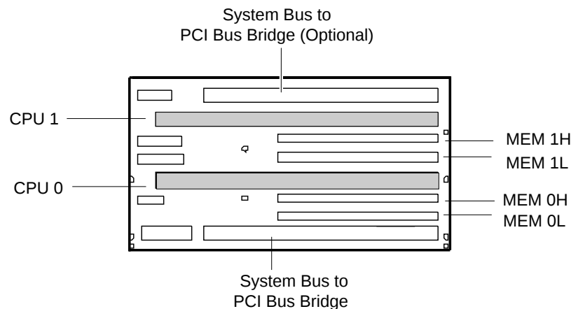
AlphaServer 4000 Motherboard
