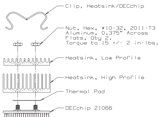
Figure D-1 Heatsink Assembly
