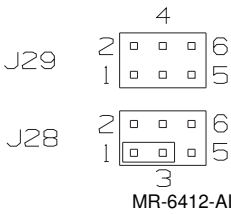
Figure 2–10 SROM Select Jumper Positions (J28 and J29)
