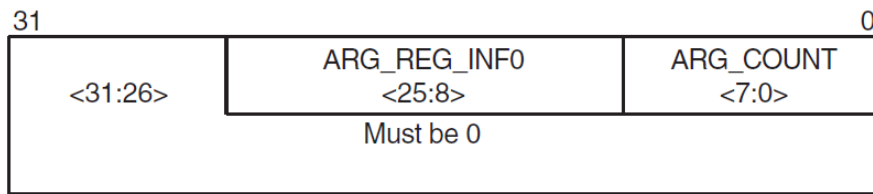
Figure 3.10. Argument Information Register (R25) Format
