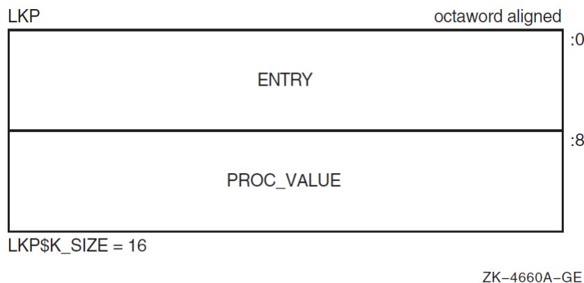
Figure 3.11. Linkage Pair Block Format
